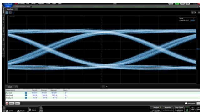
Input Signal @56Gbps
