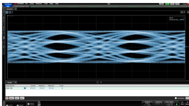
Output Signal @56Gbaud
