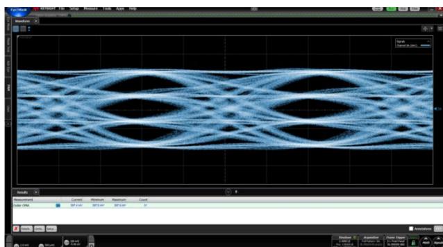
Input Signal @56Gbaud
